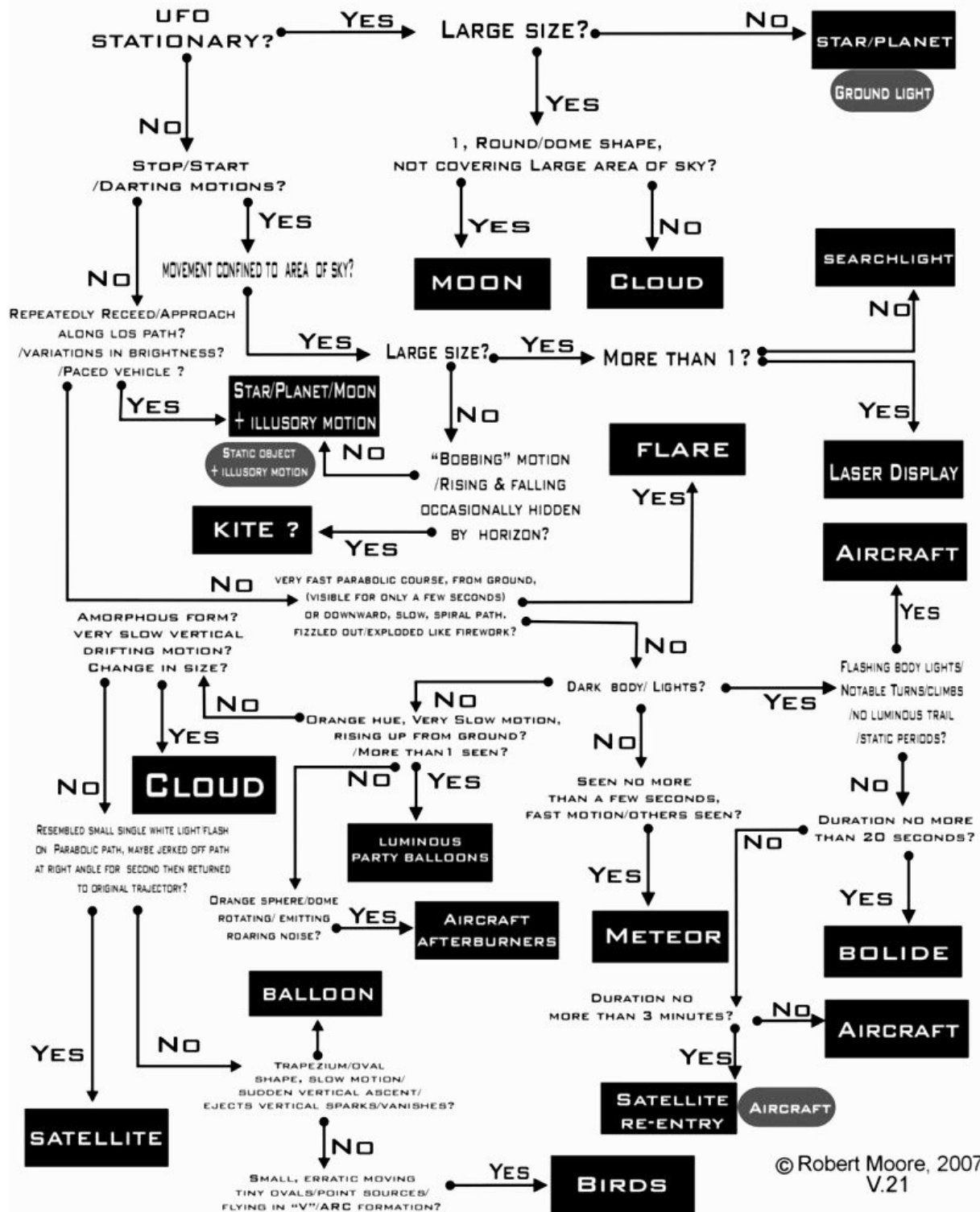
Figure 9: Flowchart depicting common nocturnal IFO types, based on described attributes. Dark blocks depict most likely, lighter boxes indicate possible but less likely causes while rounded oblongs notably uncommon options.
